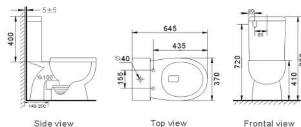
B2355A Rimless two piece toilet Size: 645x370x800 mm
