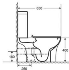
B2315A Rimless two piece toilet Size: 650x340x790 mm
