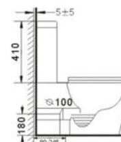
B2303A-2 Rimless two piece toilet Size: 665x360x845 mm
