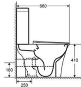
B2313A Rimless two piece toilet Size: 660x360x820 mm
