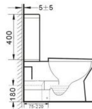
B2359A Rimless two piece toilet Size: 620x365x790 mm
