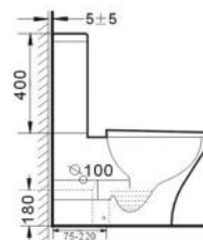
B2366A Rimless two piece toilet Size: 610x360x855 mm
