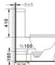
B2303A-1 Rimless two piece toilet Size: 642x380x850 mm
